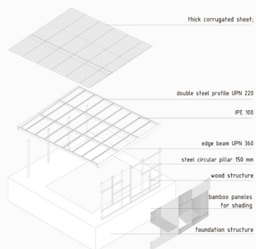
roof and radiation protection system
